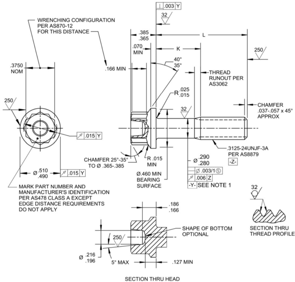
FIGURE 1 - BOLT
